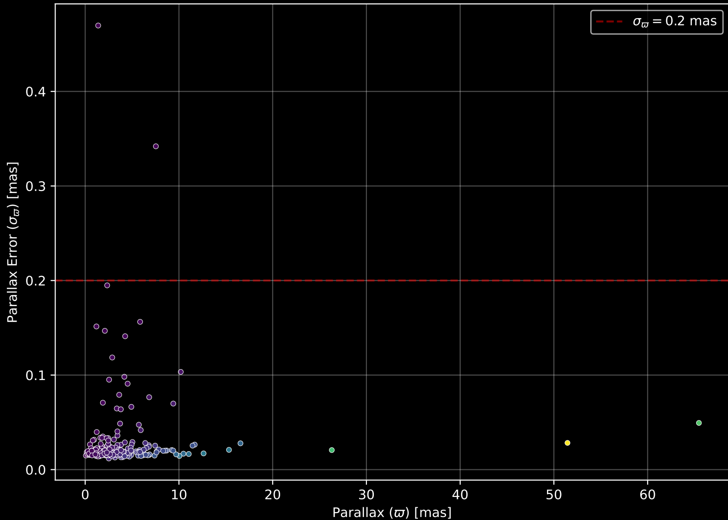
APOGEE DR17 Field: [239+50_MGA] Parallax Quality (n= 212)
