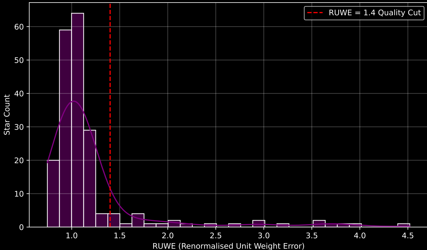
GAPOGEE DR17 Field [239+50_MGA] RUWE Distribution (n= 201)
