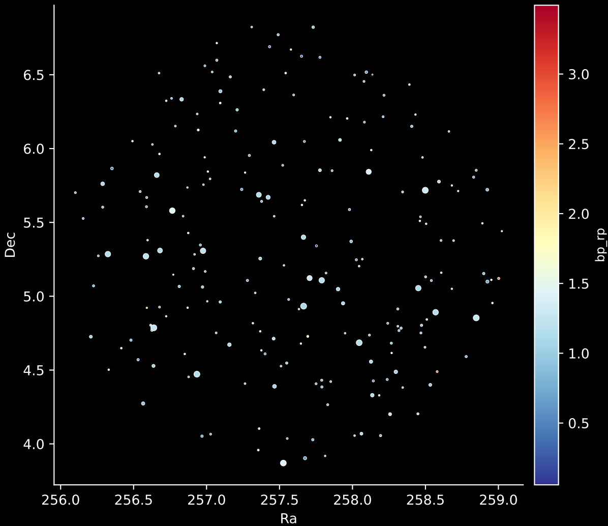
APOGEE DR17 Field: [239+50_MGA] Stars: 212
